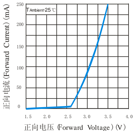
Volt-Ampere Characteristics
